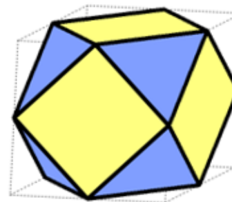
Kubo-Oktaeder
